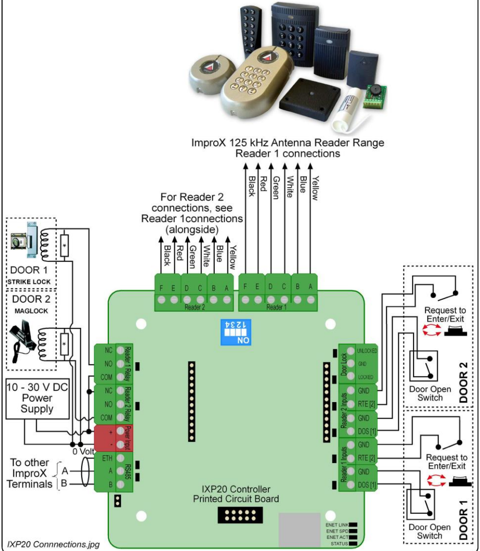
Figure 4: Typical IXP20 Controller Electrical Connections
